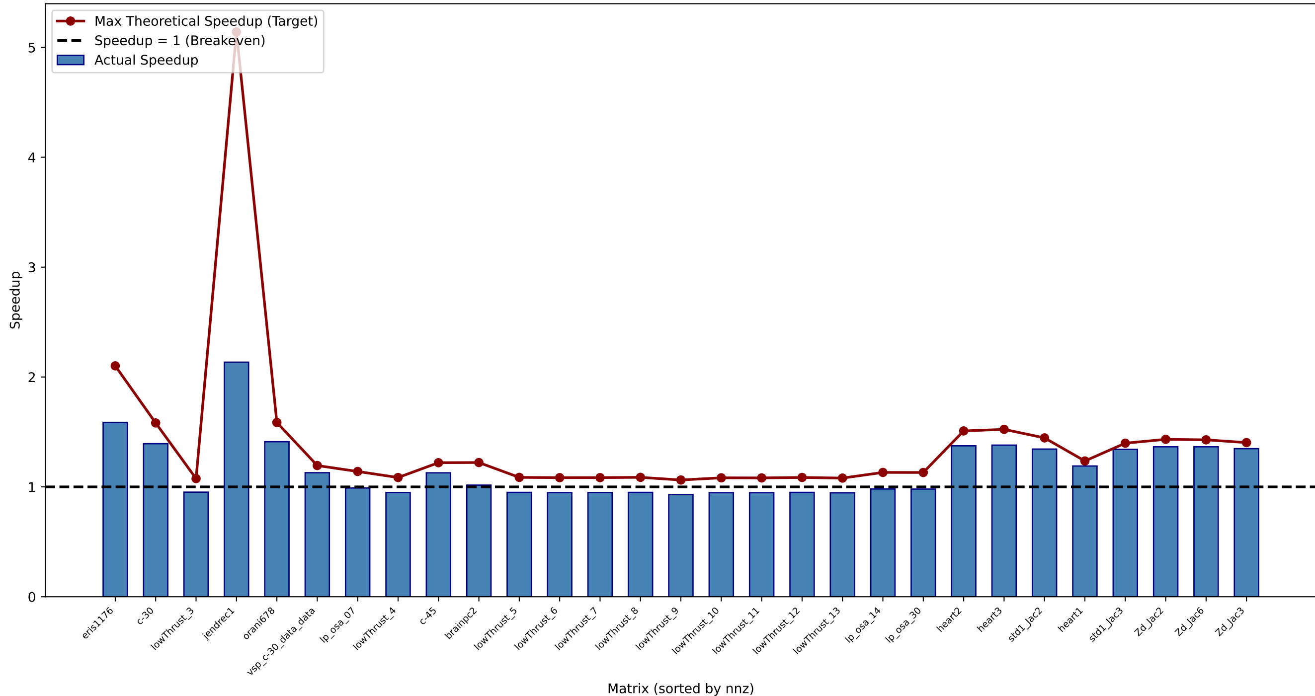
SpMM Speedups: dense=mkl, sparse=naive (Line: Max Theoretical Target, Bars: Actual Achieved)
