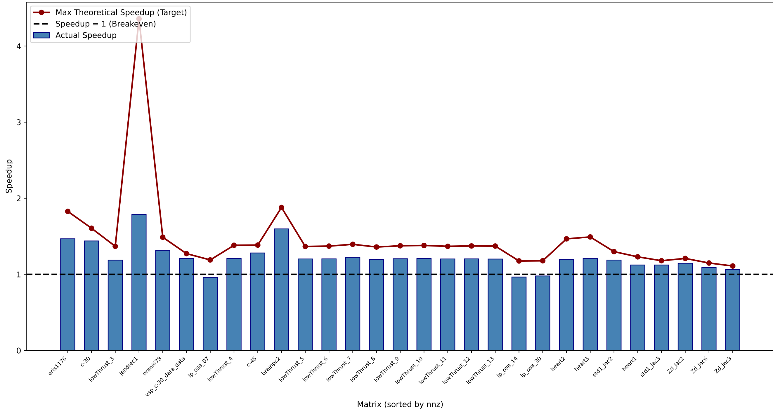
SpMV Speedups: dense=blas, sparse=uzp (Line: Max Theoretical Target, Bars: Actual Achieved)
