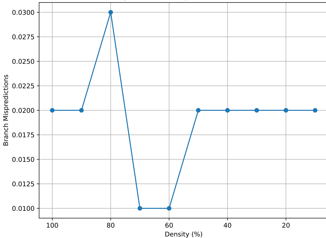
Matrix Density vs Branch Mispredictions (Sieber - consec)
