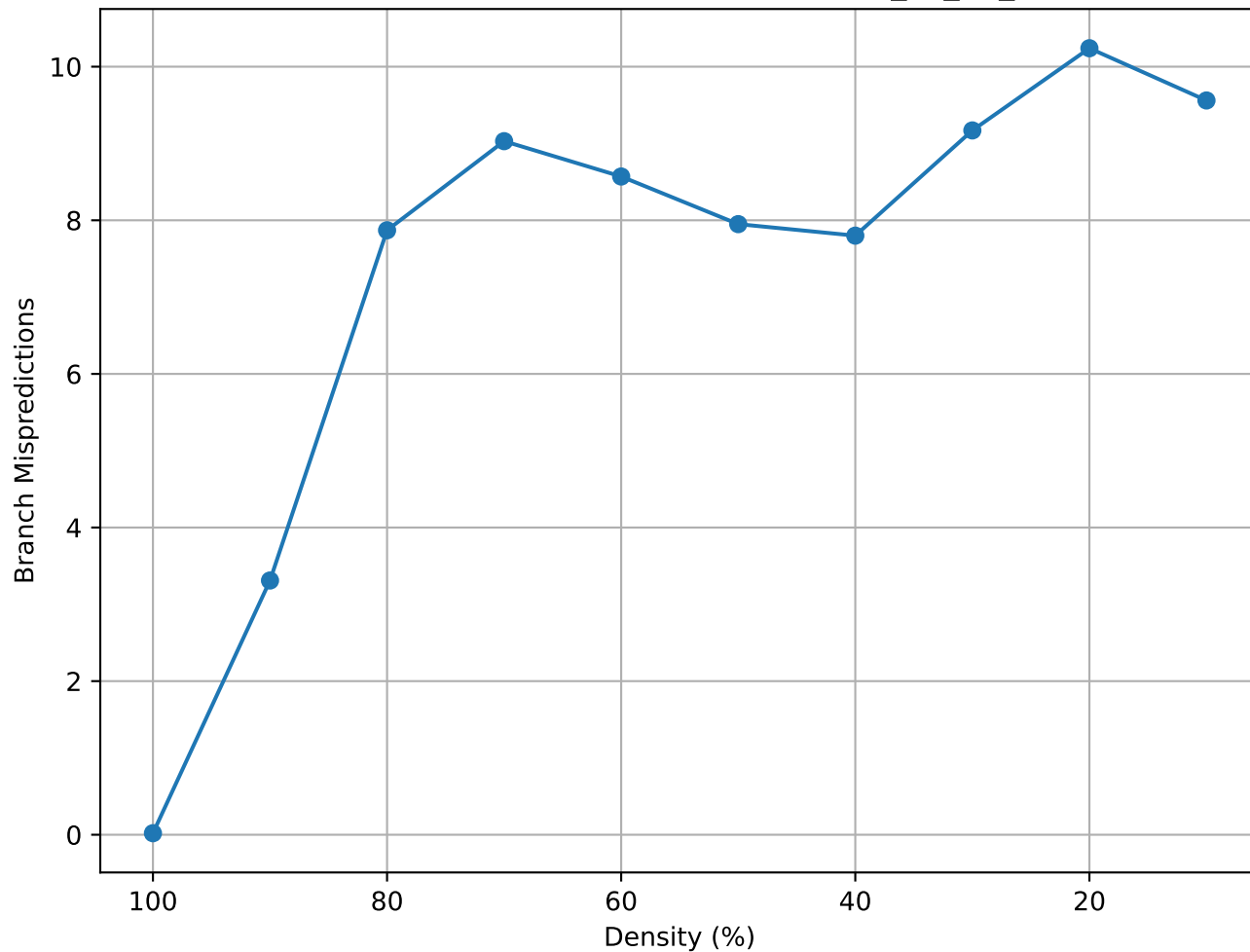
Matrix Density vs Branch Mispredictions (TSOPF_FS_b9_c6 - random)
