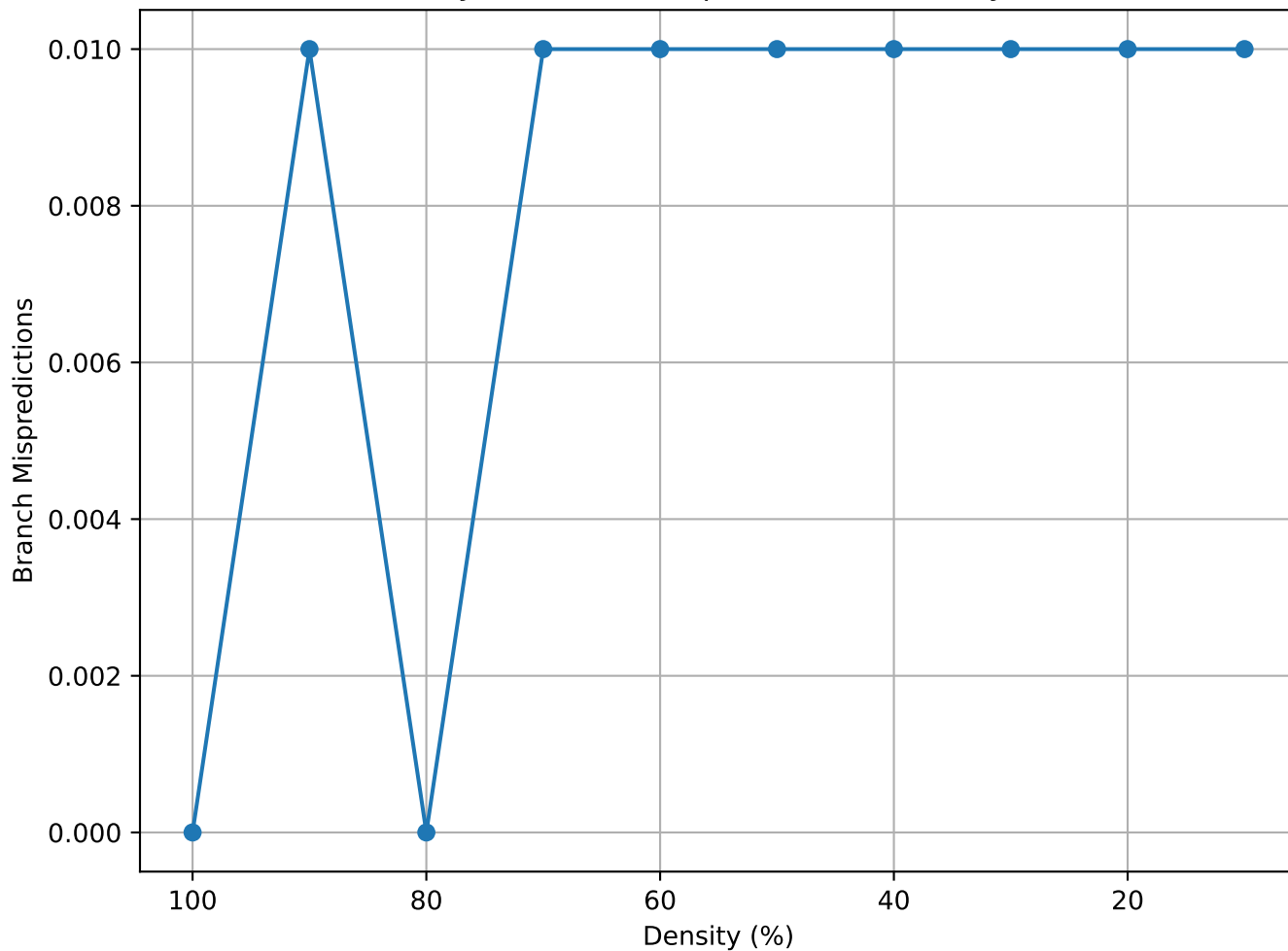
Matrix Density vs Branch Mispredictions (bloweybl - consec)
