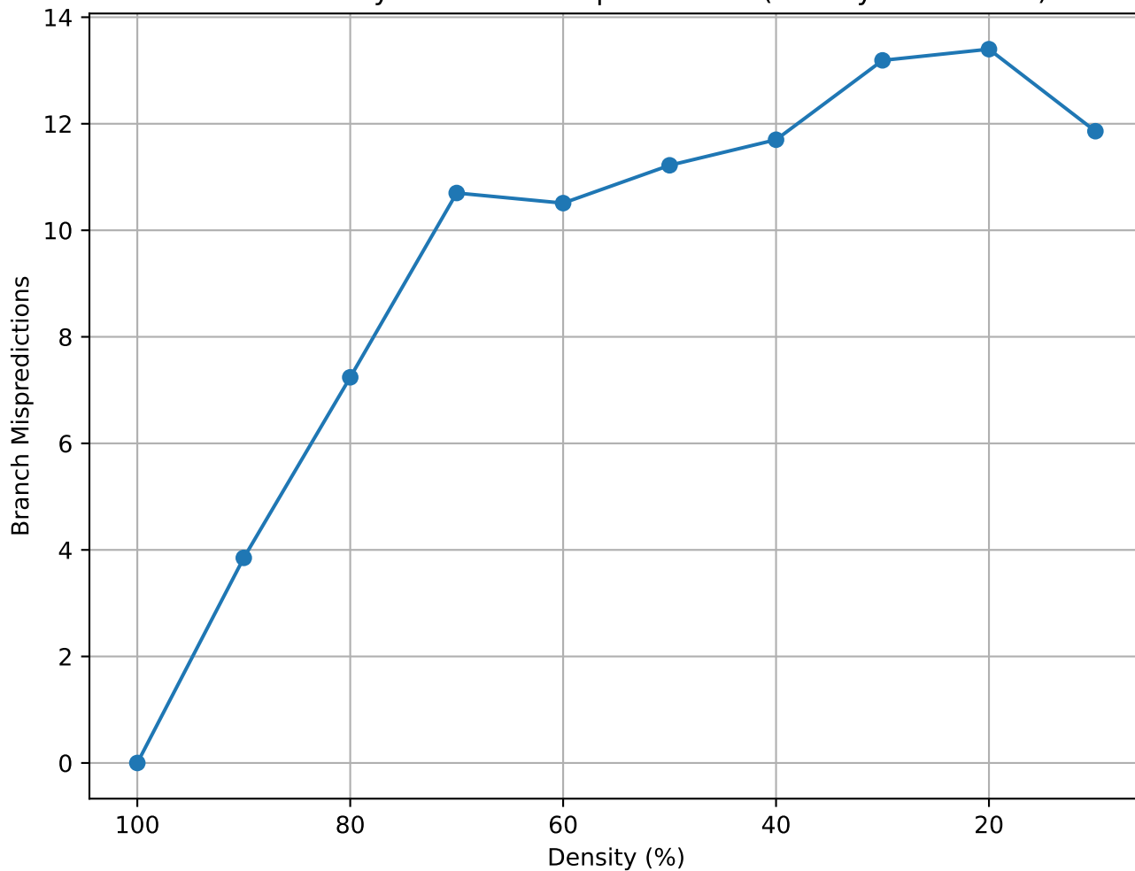
Matrix Density vs Branch Mispredictions (bloweybl - random)
