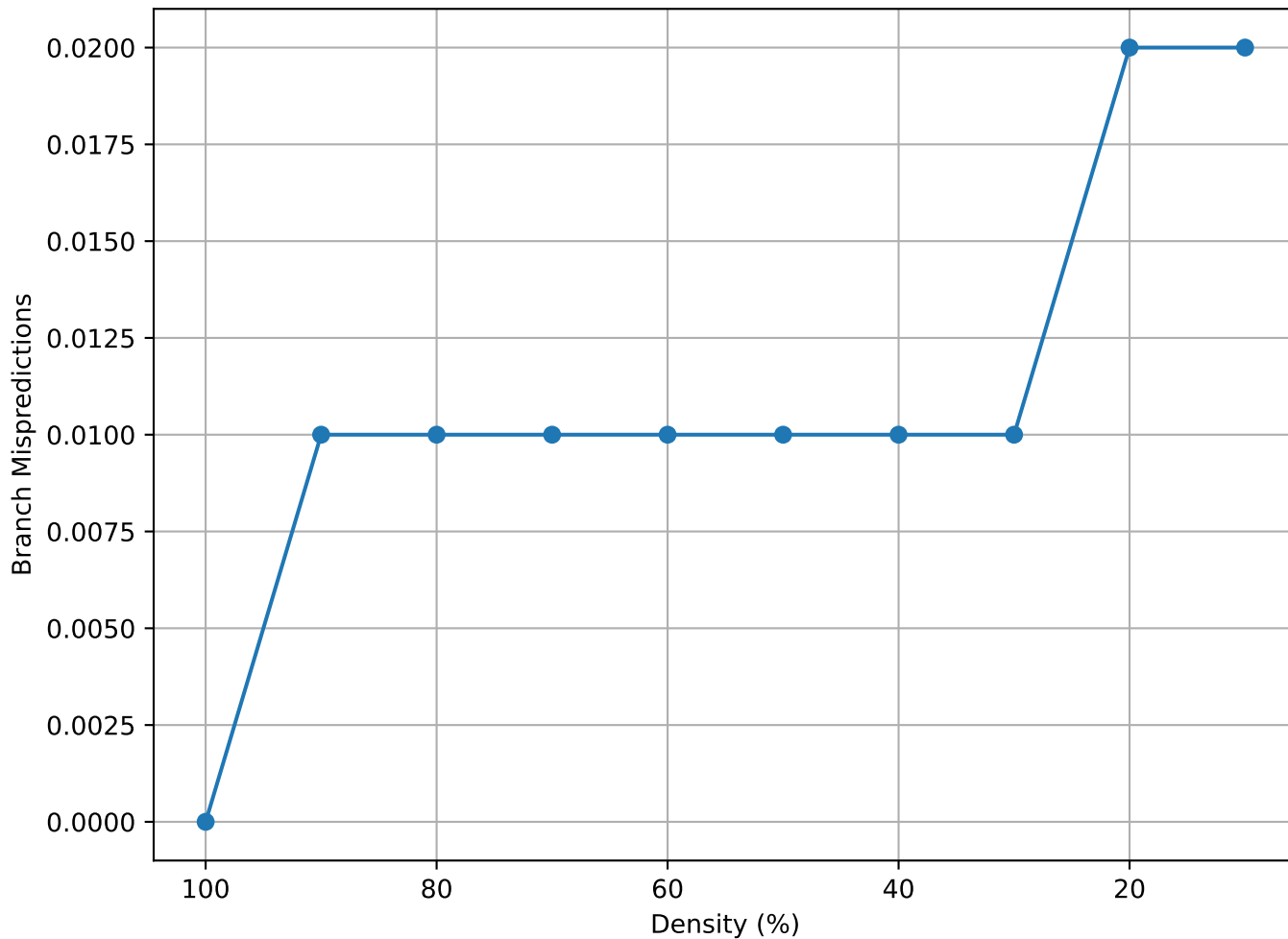
Matrix Density vs Branch Mispredictions (bloweybl - truncated)
