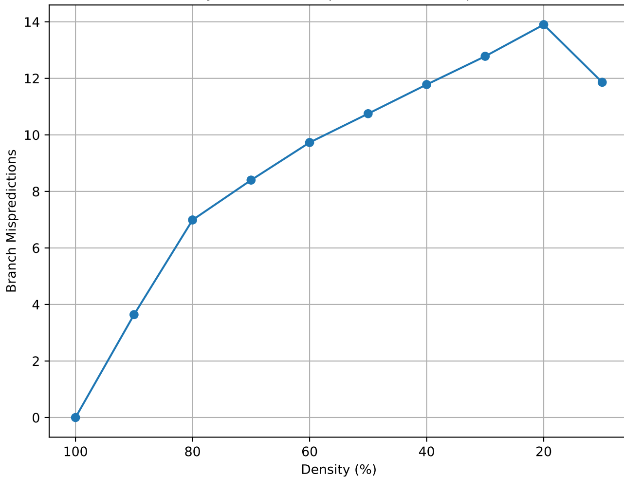
Matrix Density vs Branch Mispredictions (brainpc2 - random)
