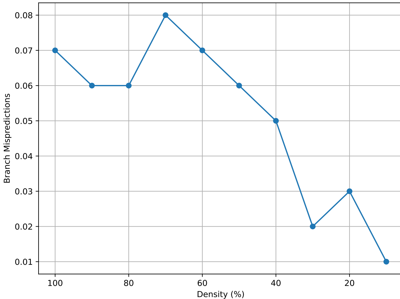
Matrix Density vs Branch Mispredictions (c-30 - consec)
