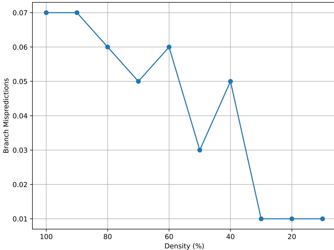
Matrix Density vs Branch Mispredictions (c-30 - truncated)
