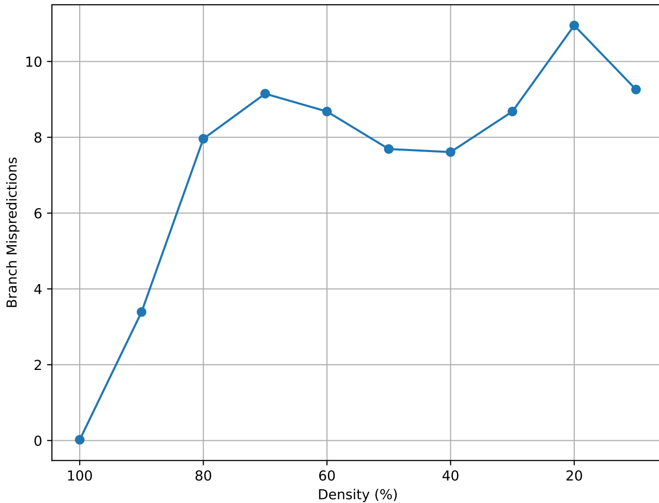
Matrix Density vs Branch Mispredictions (case9 - random)
