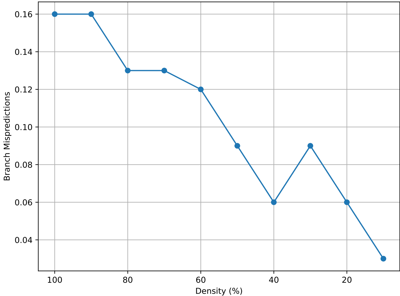
Matrix Density vs Branch Mispredictions (cz2548 - consec)
