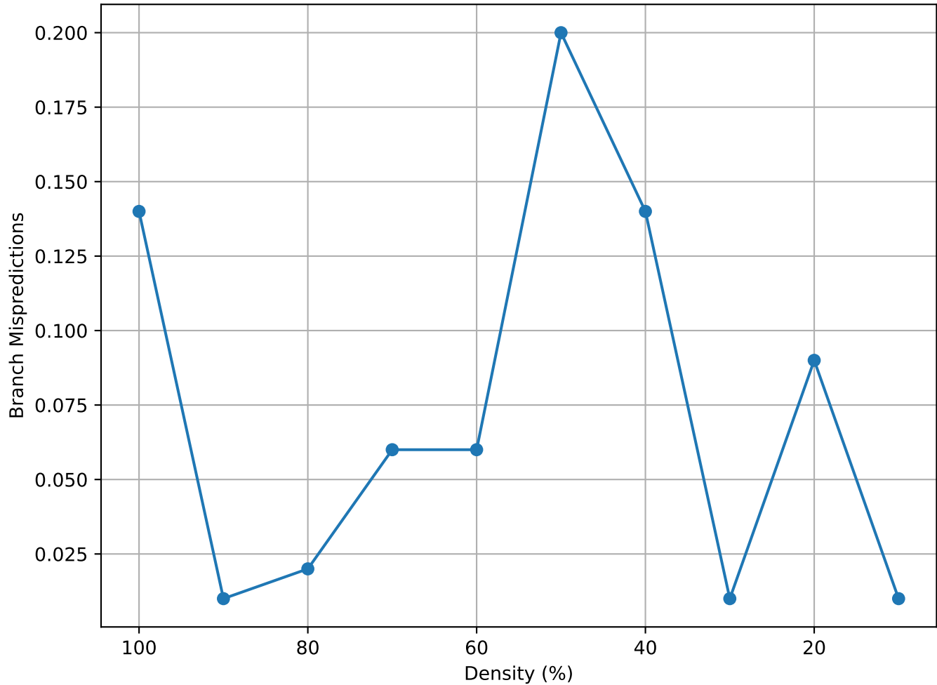
Matrix Density vs Branch Mispredictions (cz2548 - random)
