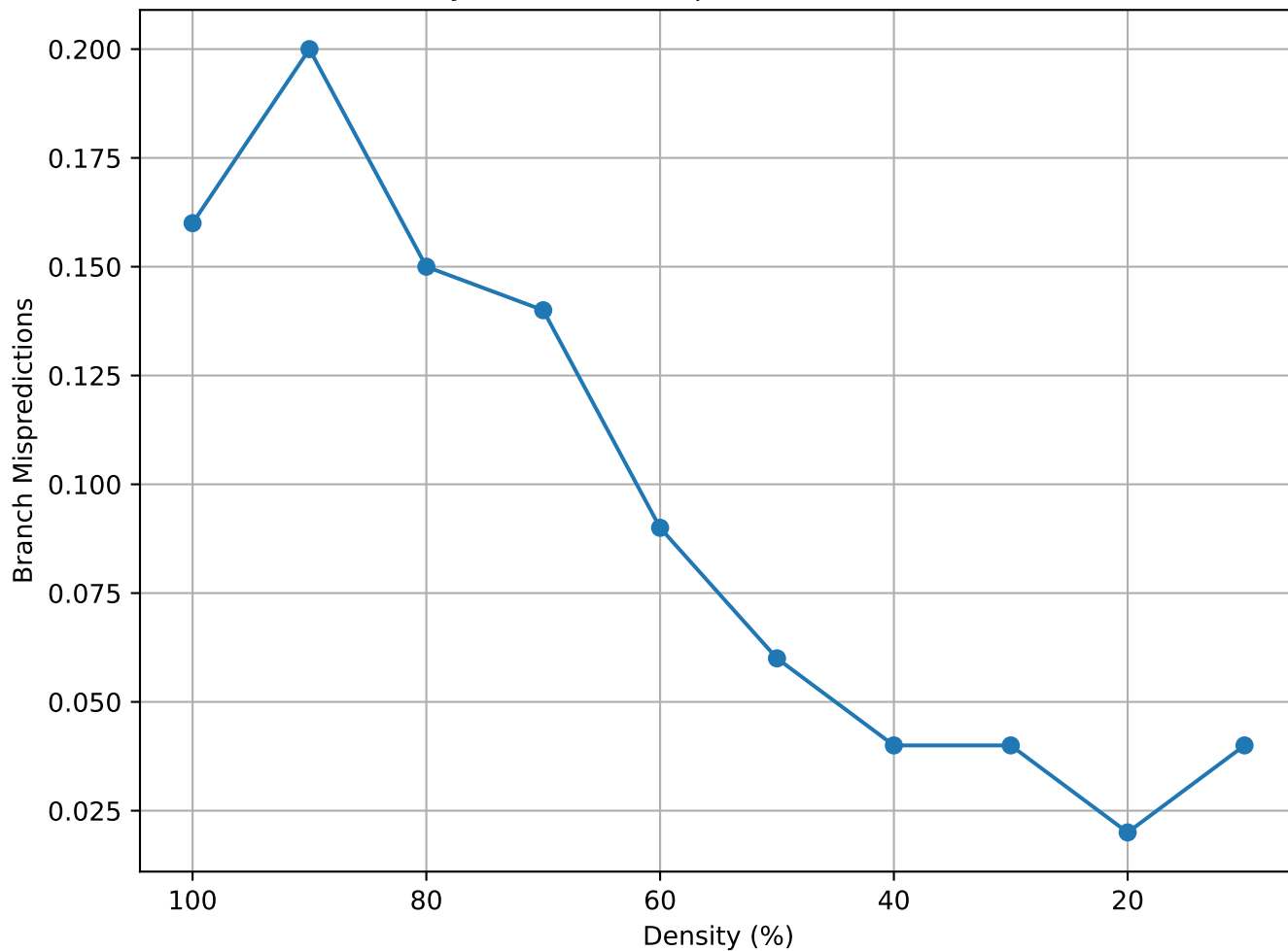
Matrix Density vs Branch Mispredictions (cz2548 - truncated)
