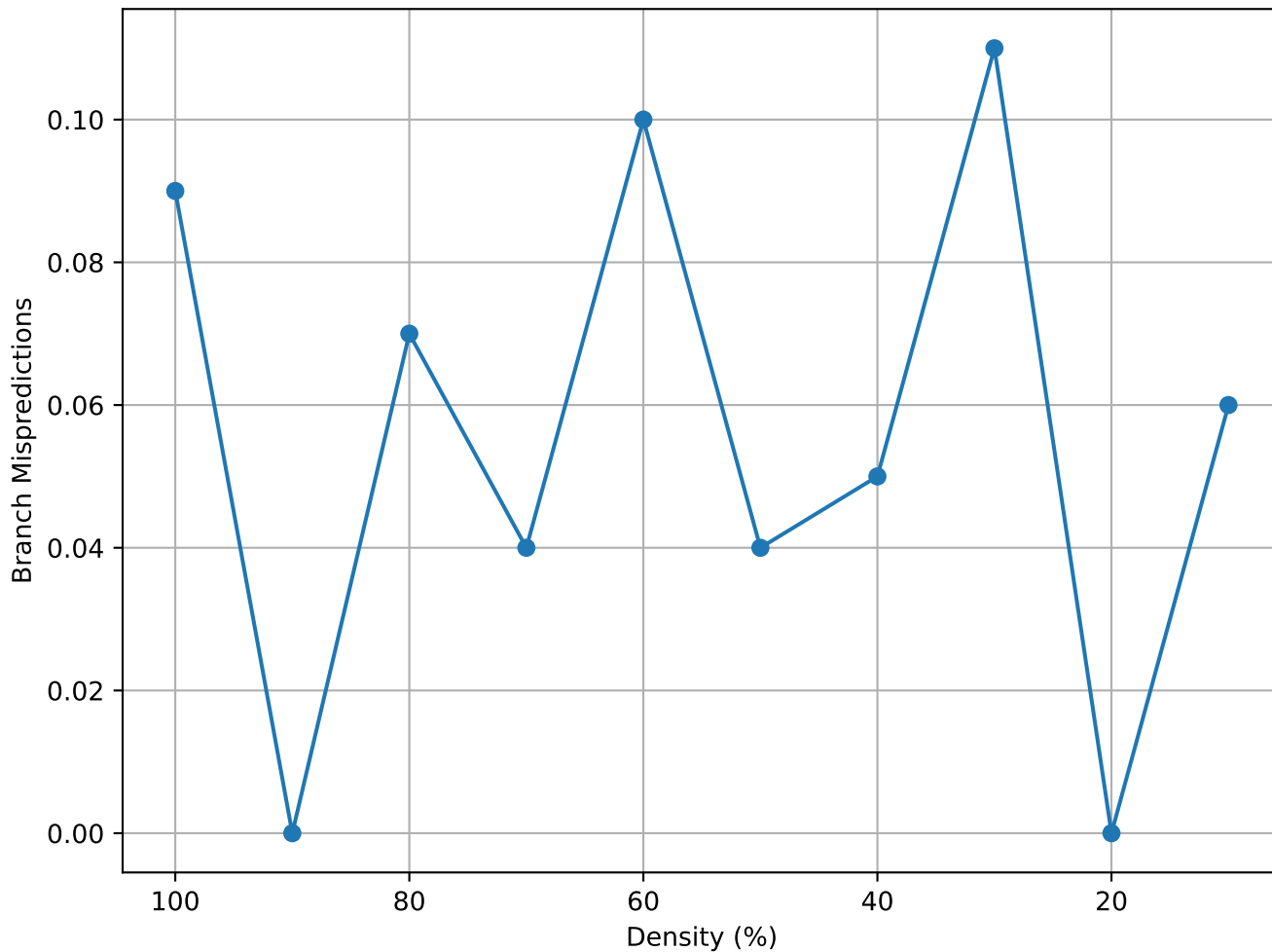
Matrix Density vs Branch Mispredictions (eris1176 - random)
