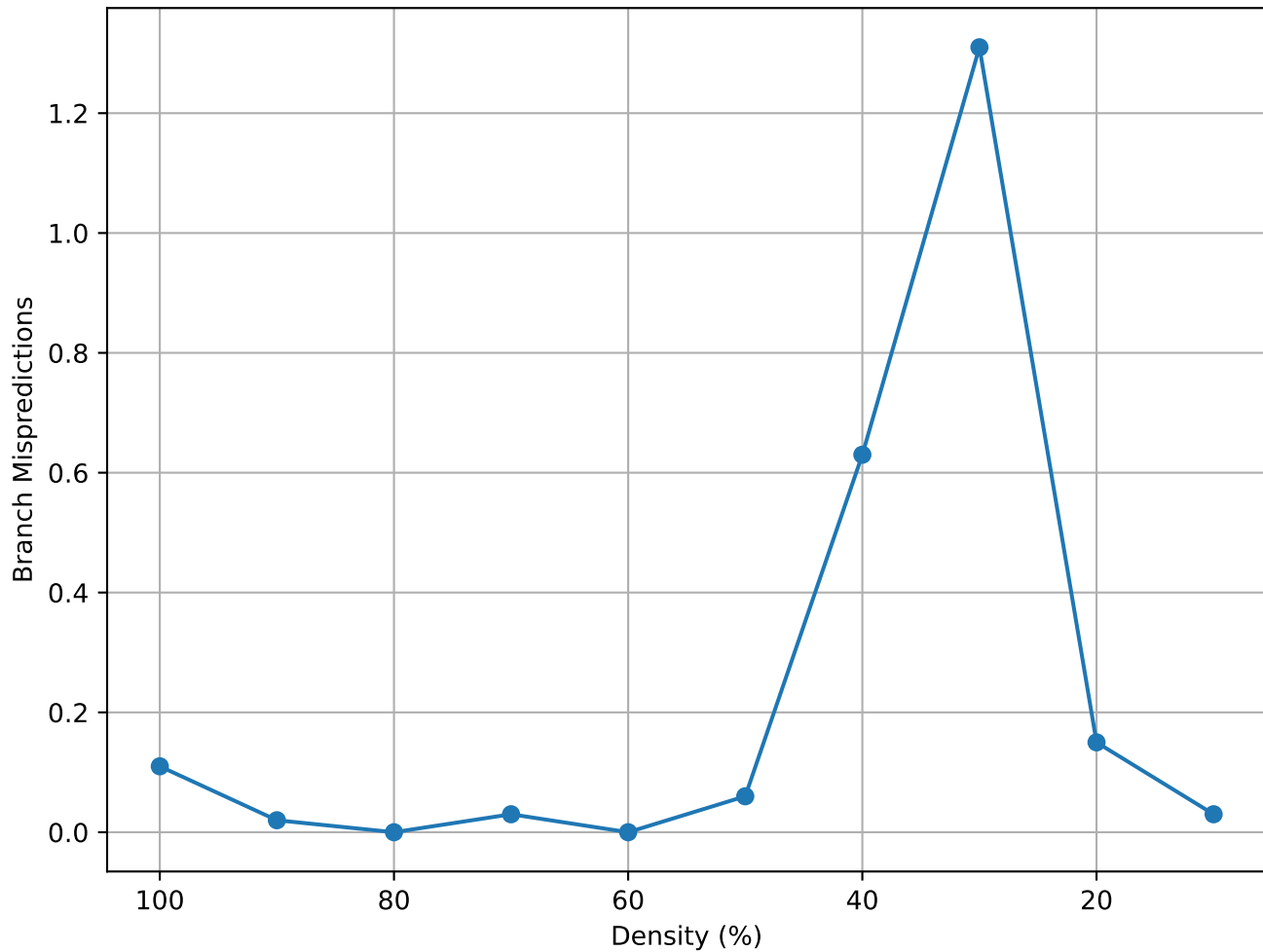
Matrix Density vs Branch Mispredictions (ex10hs - random)
