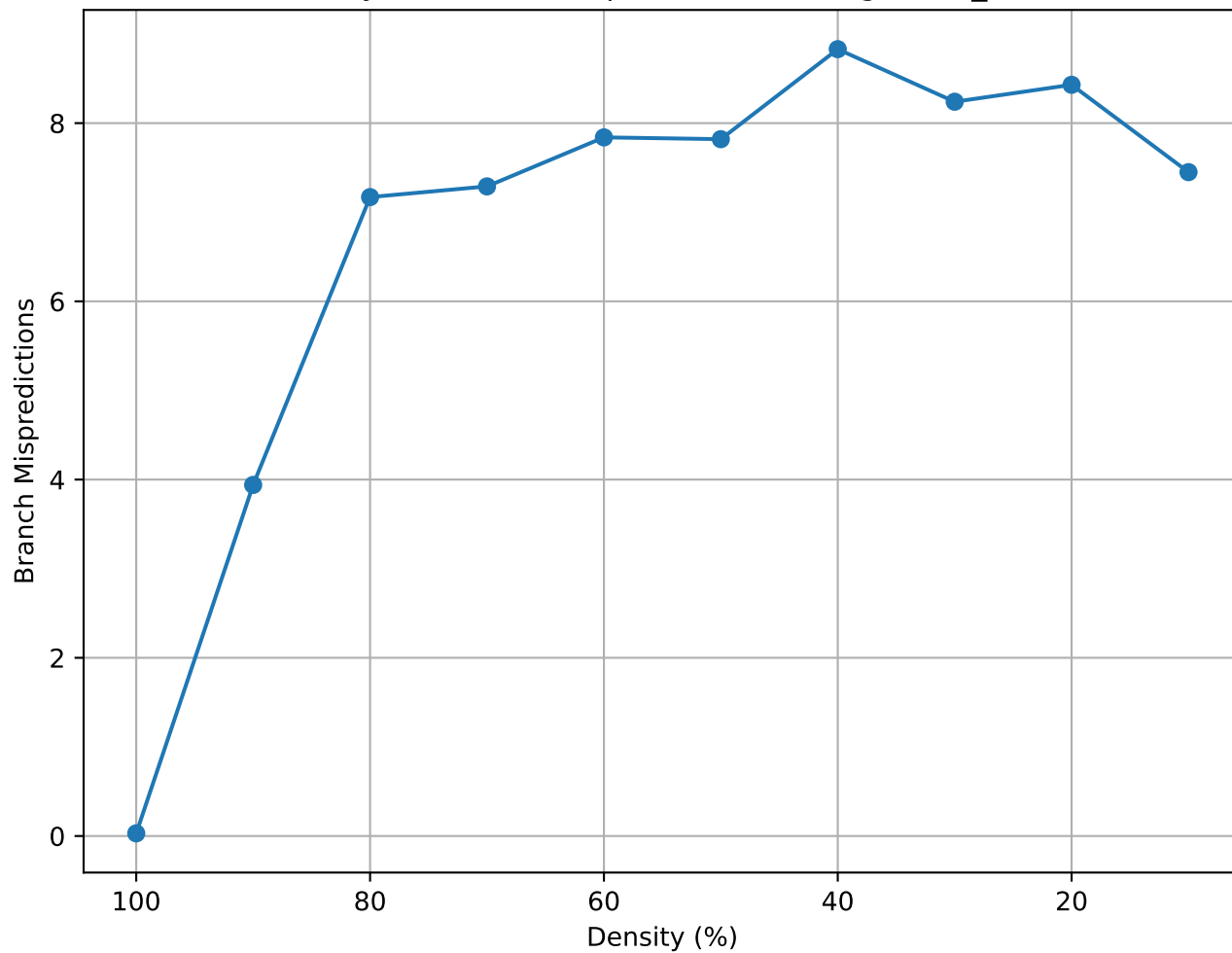
Matrix Density vs Branch Mispredictions (hangGlider_3 - random)
