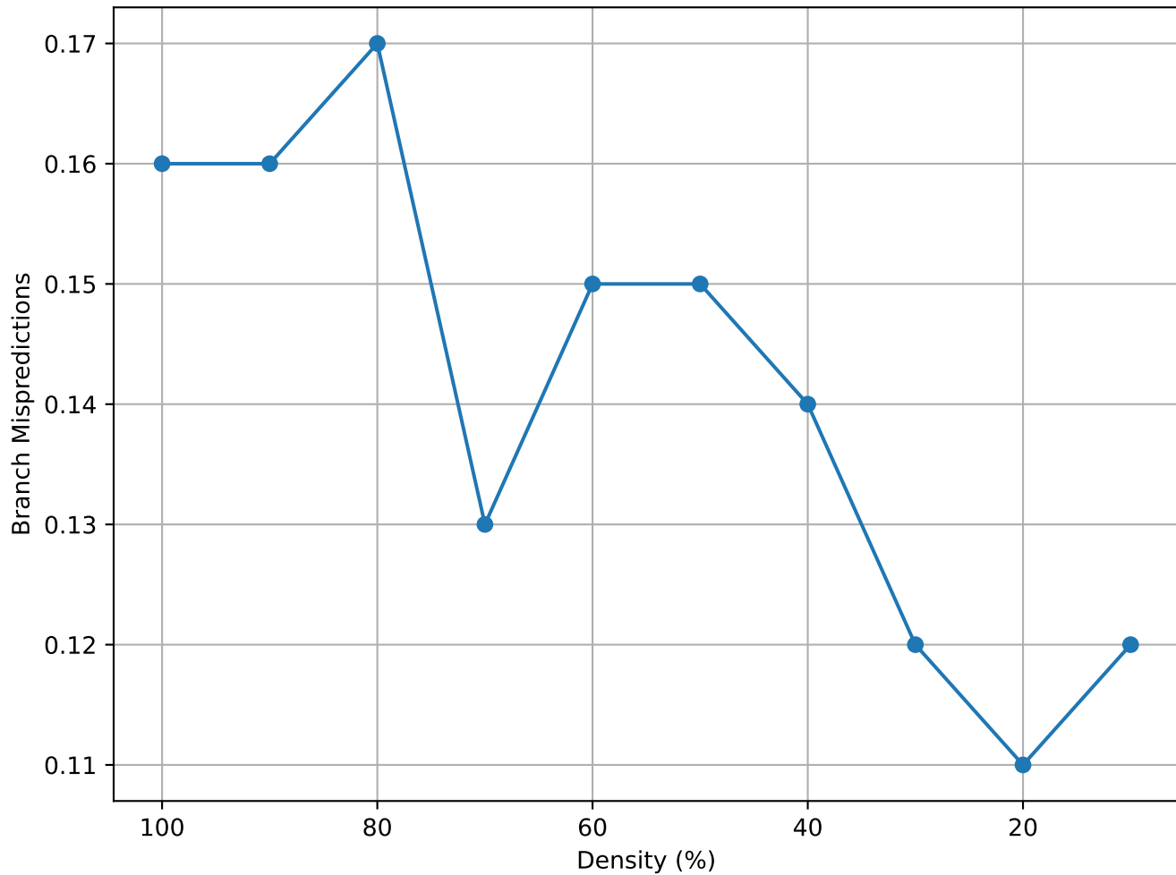
Matrix Density vs Branch Mispredictions (hangGlider_4 - consec)
