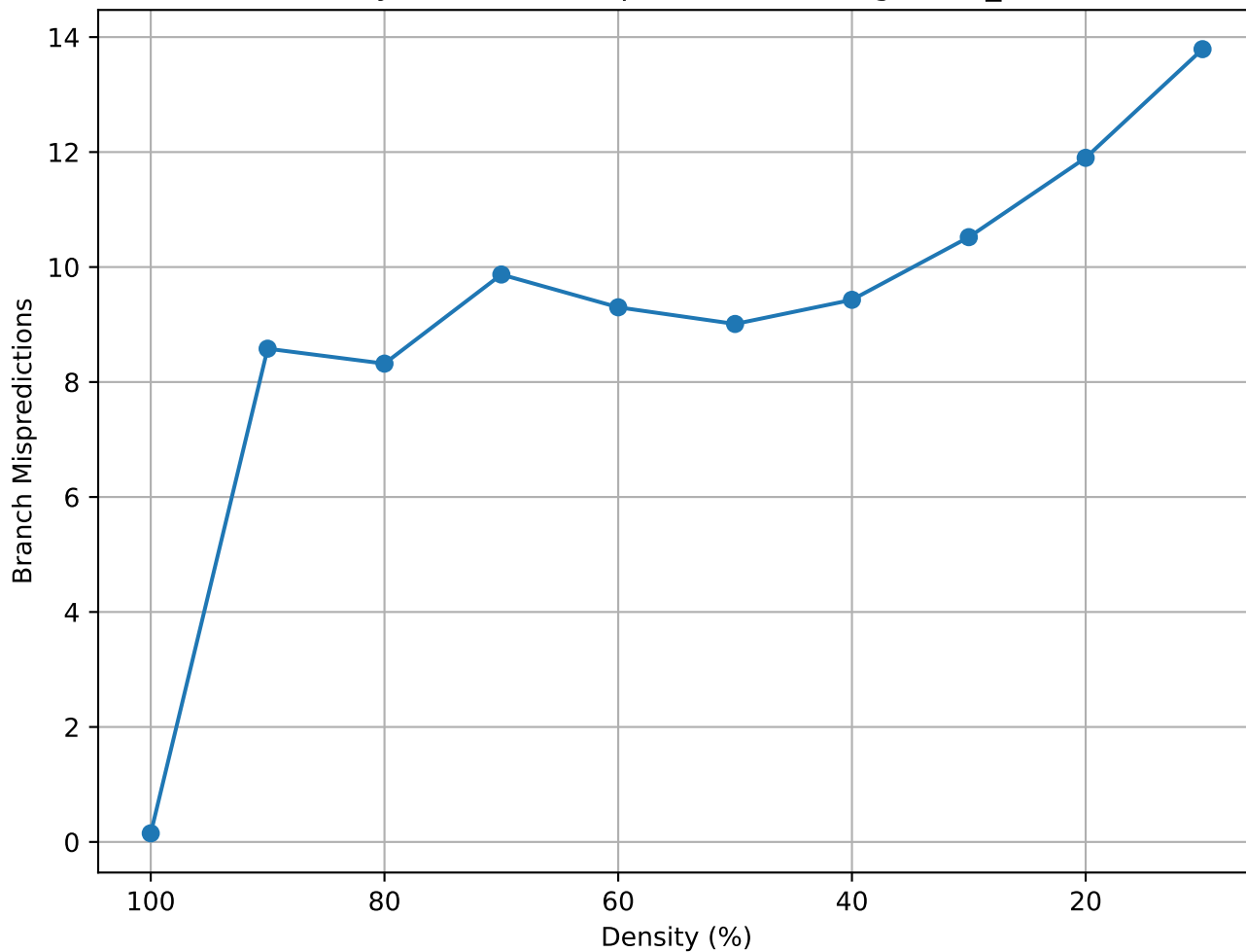
Matrix Density vs Branch Mispredictions (hangGlider_5 - random)
