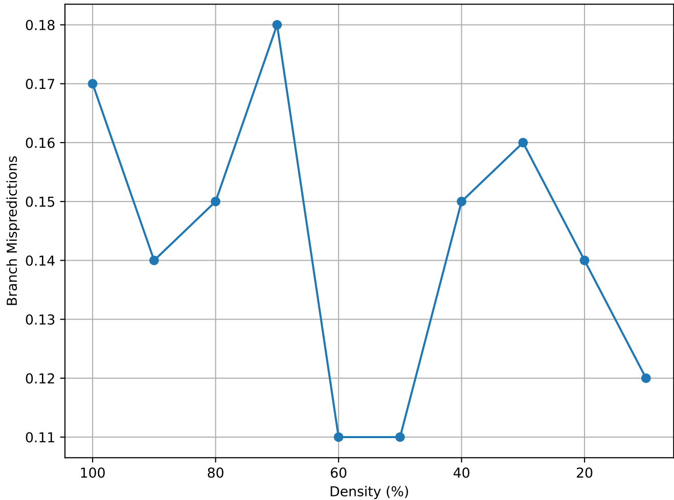
Matrix Density vs Branch Mispredictions (heart1 - consec)
