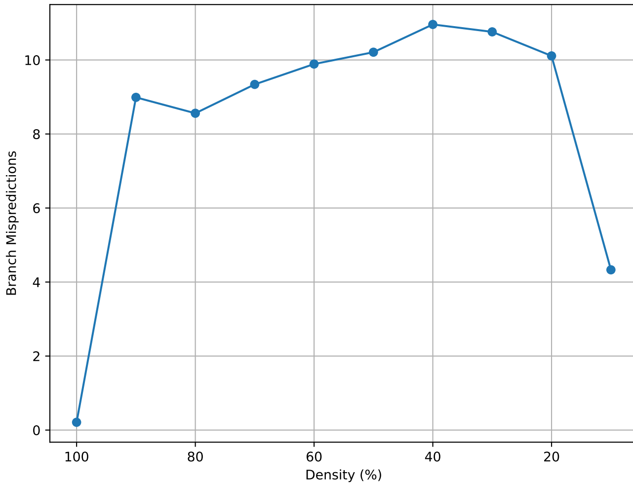
Matrix Density vs Branch Mispredictions (heart1 - random)
