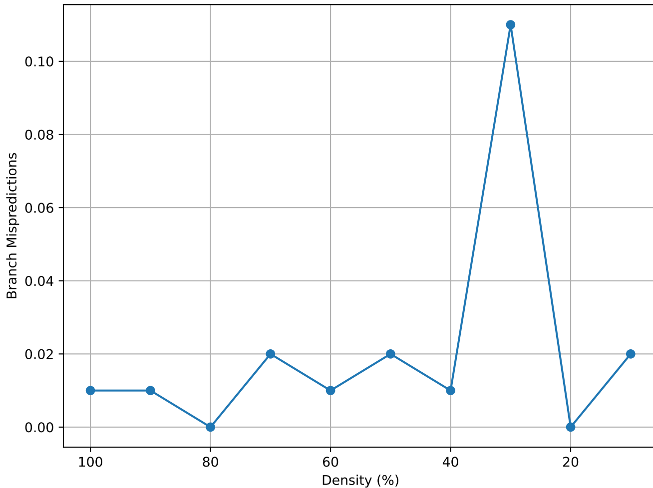
Matrix Density vs Branch Mispredictions (jendrec1 - random)
