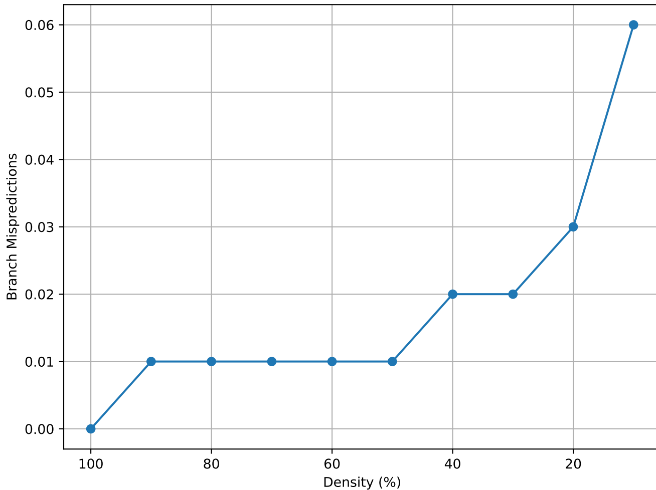
Matrix Density vs Branch Mispredictions (jendrec1 - truncated)
