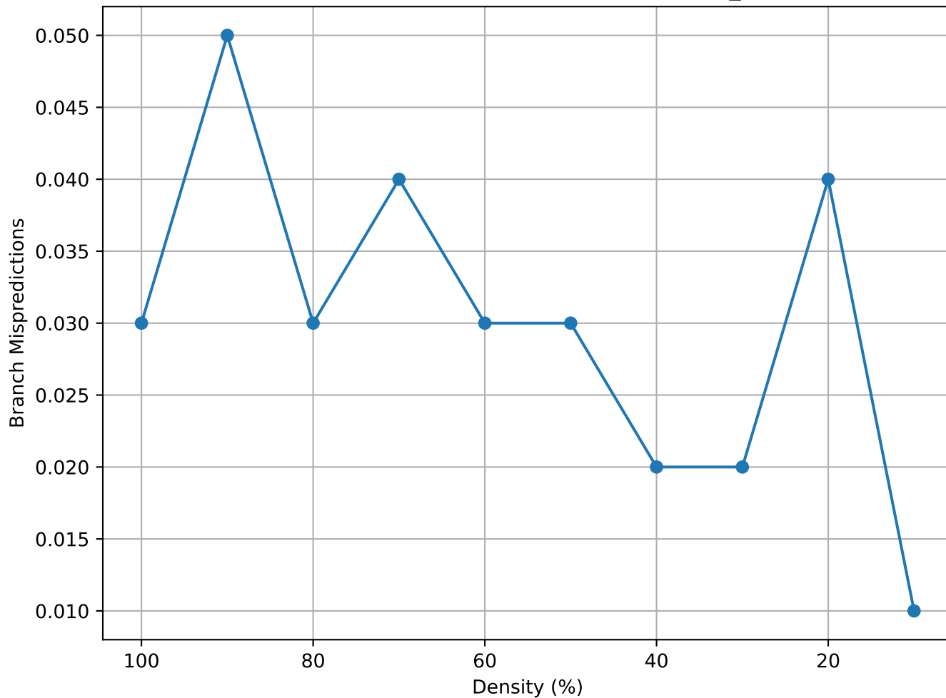
Matrix Density vs Branch Mispredictions (lowThrust_10 - truncated)
