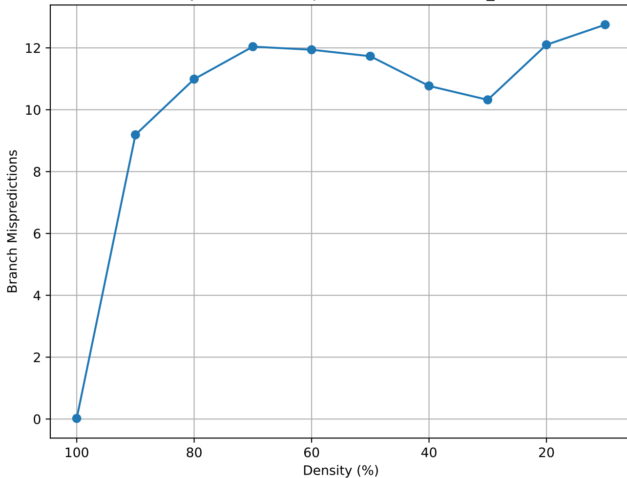
Matrix Density vs Branch Mispredictions (lowThrust_11 - random)
