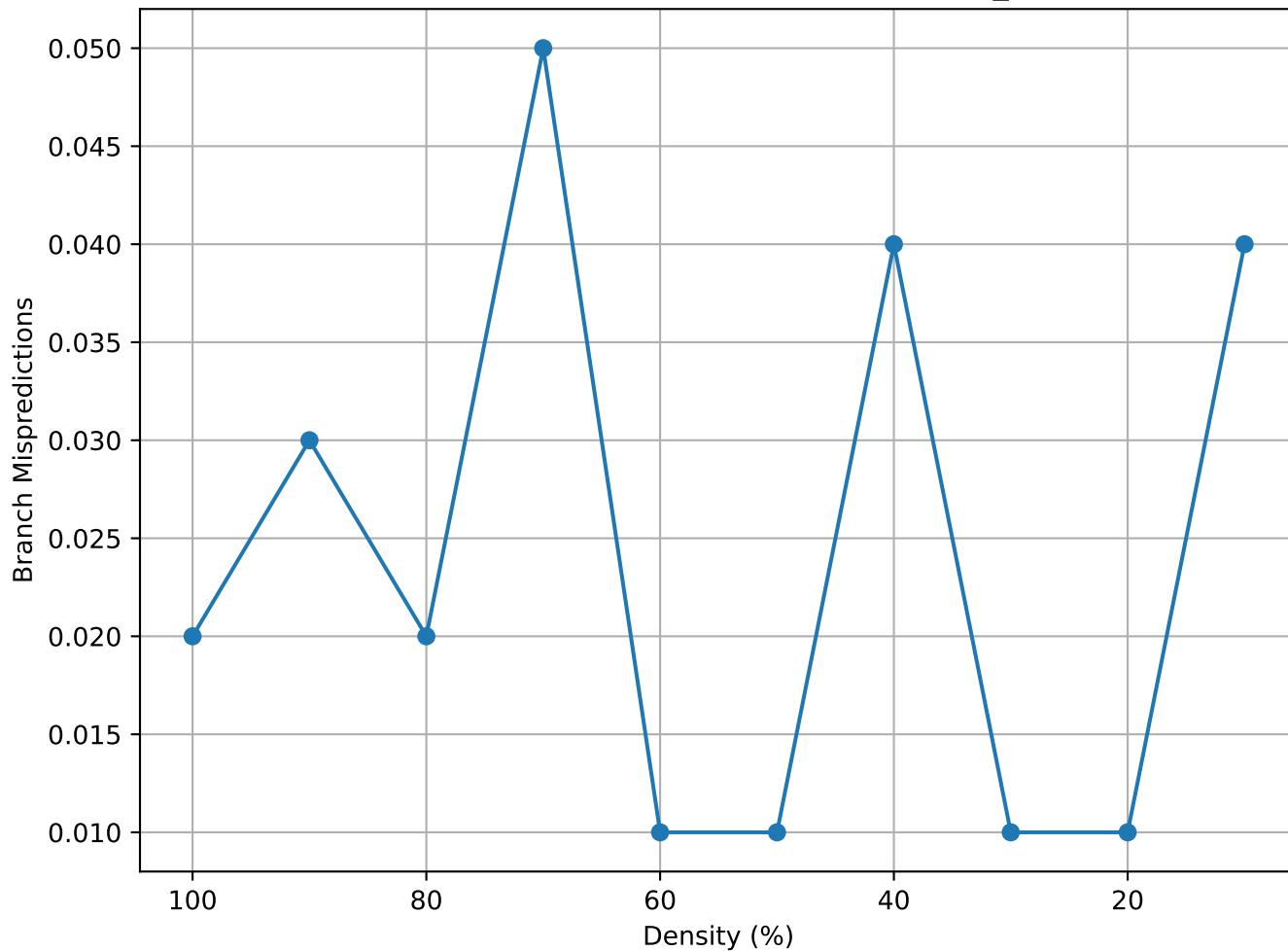
Matrix Density vs Branch Mispredictions (lowThrust_11 - truncated)
