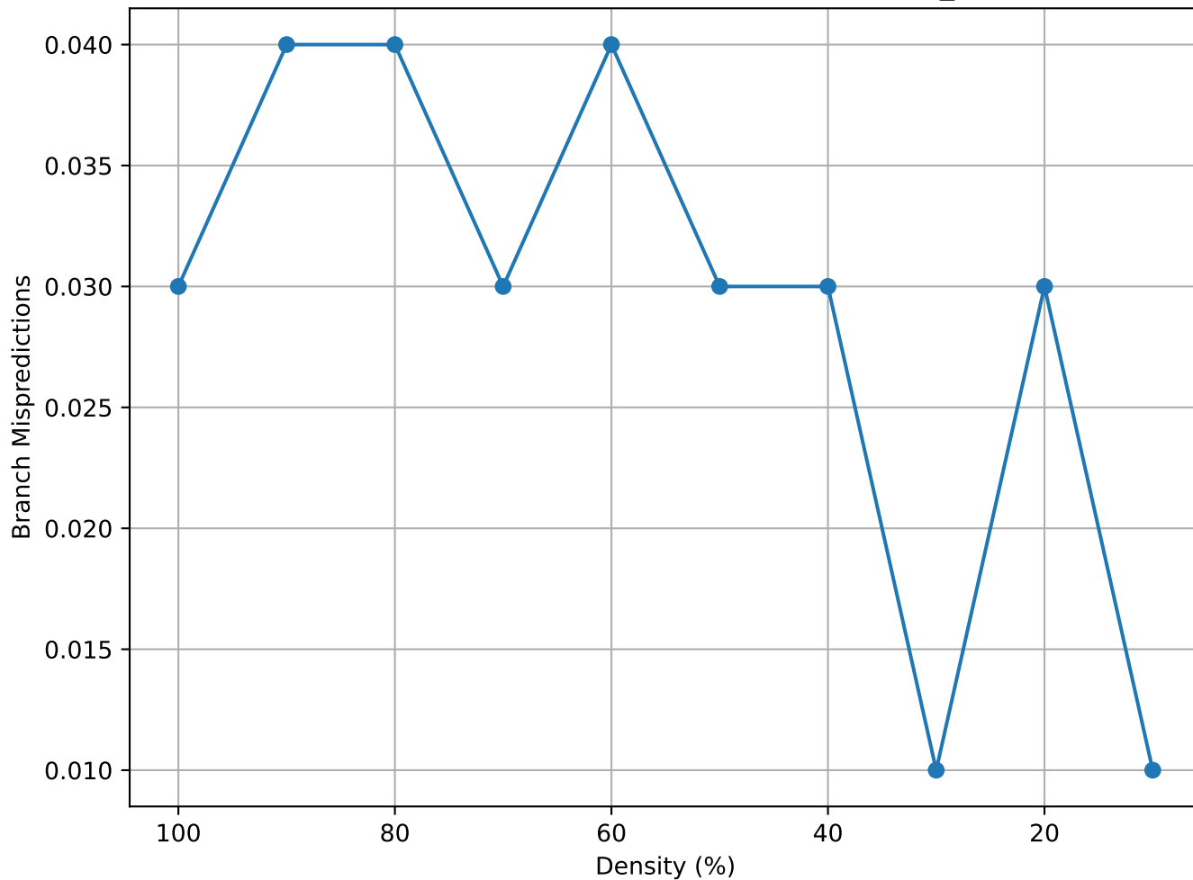
Matrix Density vs Branch Mispredictions (lowThrust_12 - consec)
