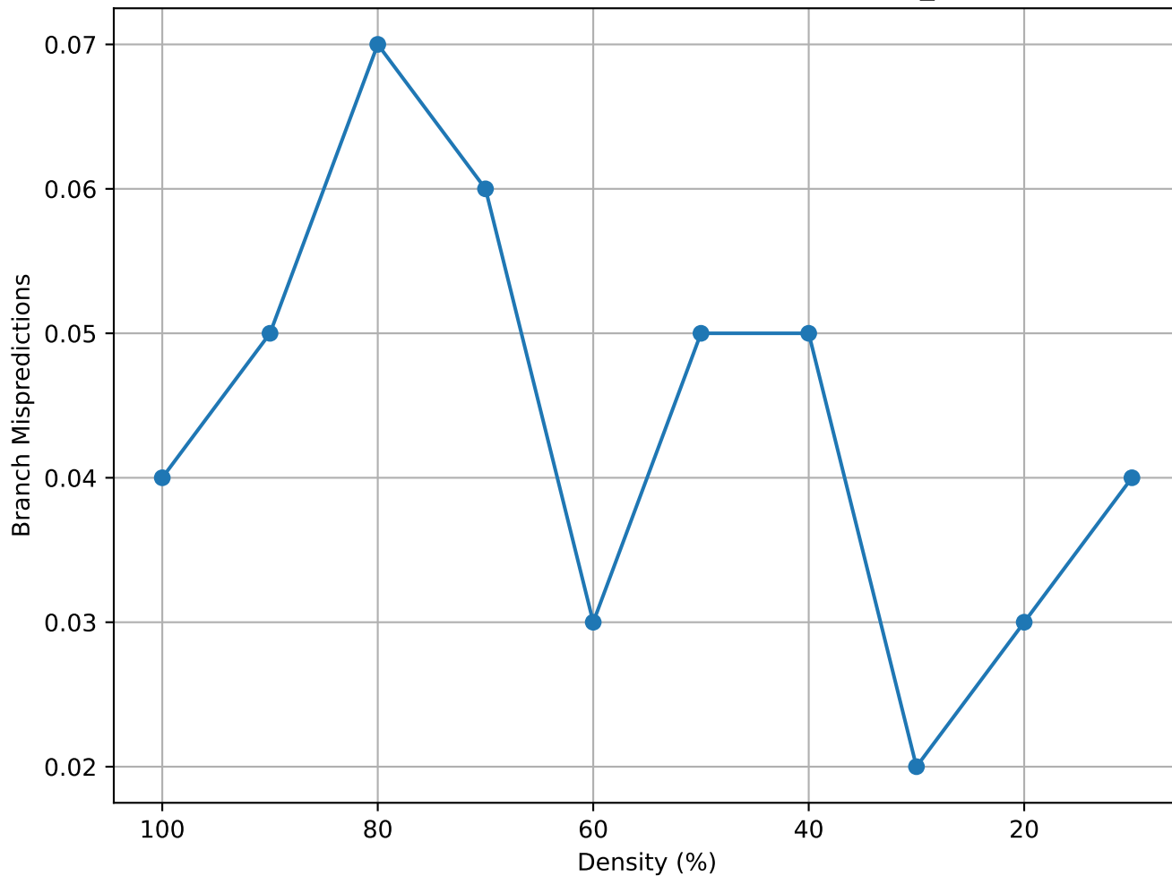
Matrix Density vs Branch Mispredictions (lowThrust_13 - consec)
