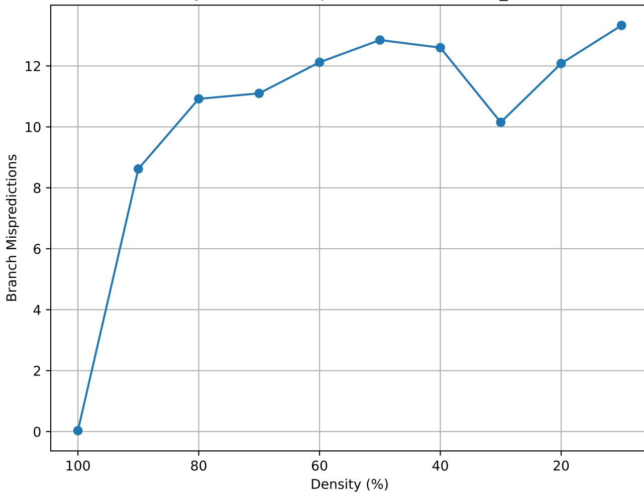
Matrix Density vs Branch Mispredictions (lowThrust_13 - random)
