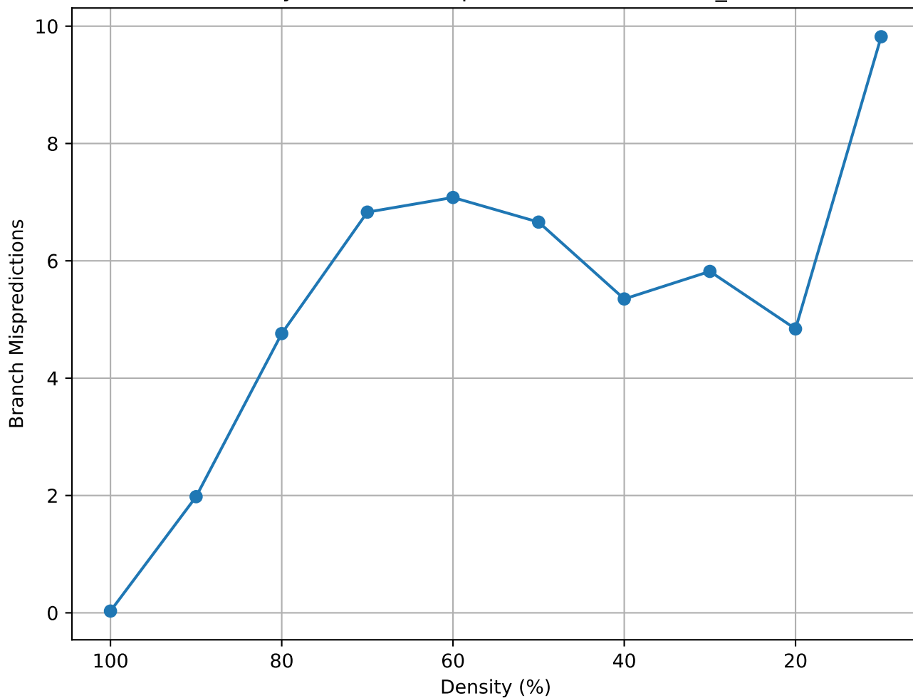
Matrix Density vs Branch Mispredictions (lowThrust_3 - random)
