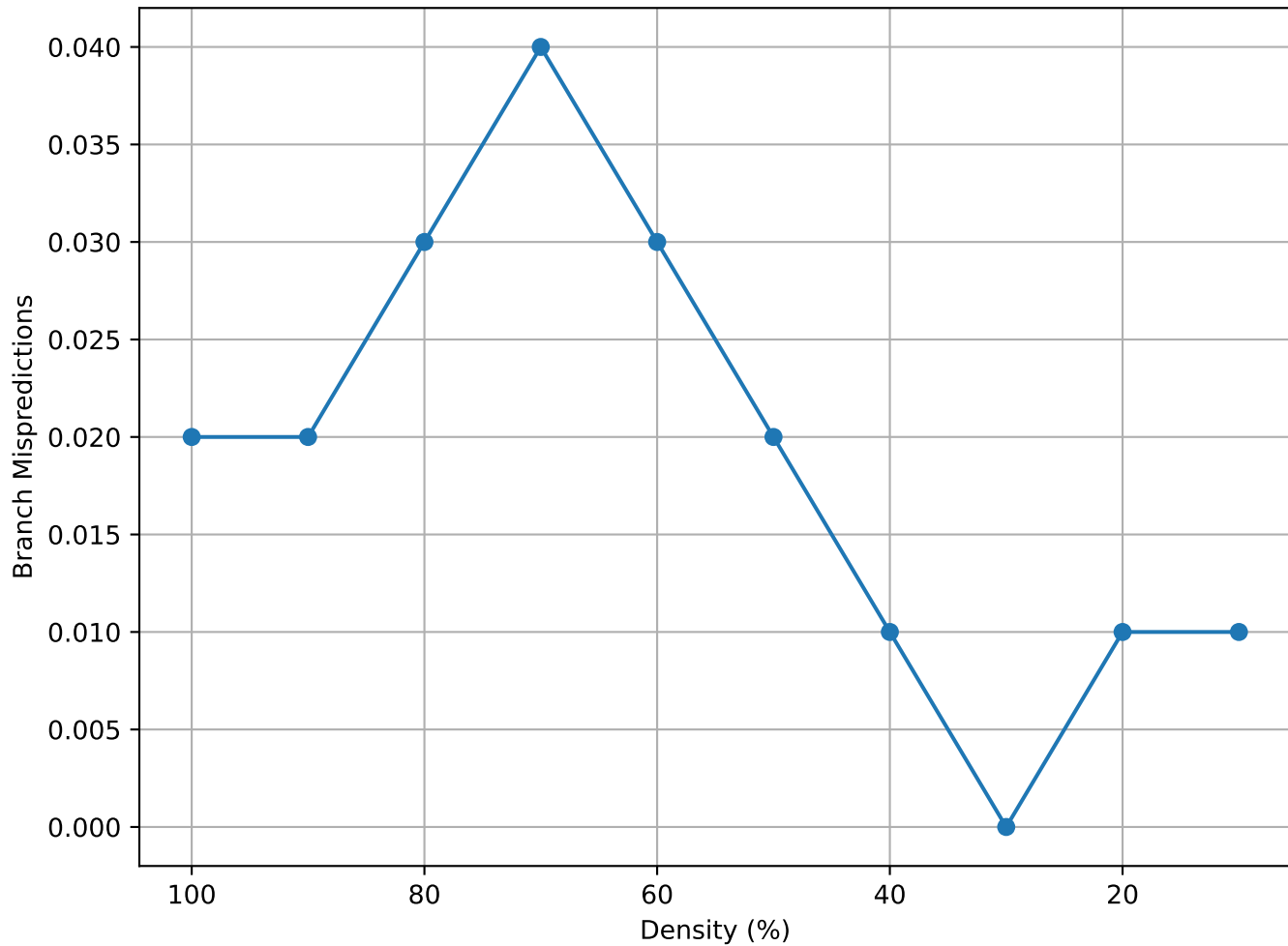
Matrix Density vs Branch Mispredictions (lowThrust_5 - truncated)
