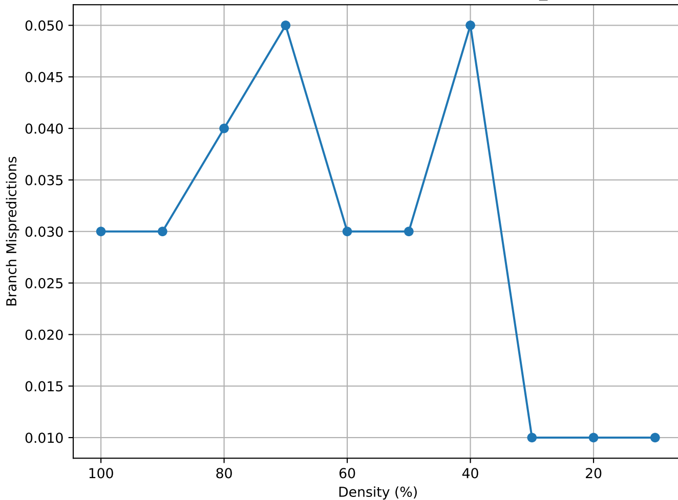
Matrix Density vs Branch Mispredictions (lowThrust_6 - consec)
