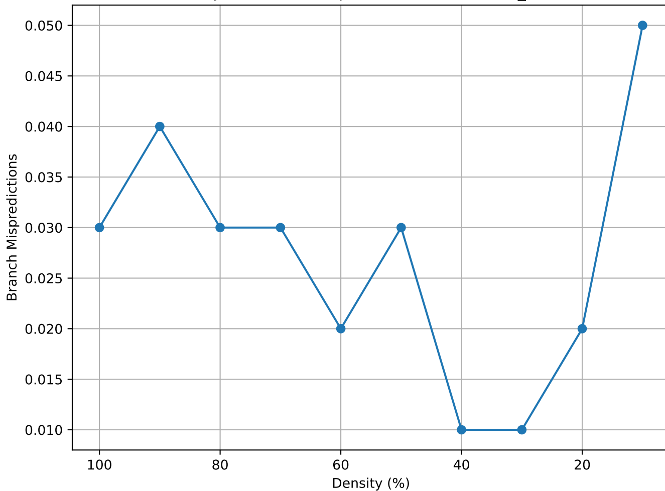
Matrix Density vs Branch Mispredictions (lowThrust_6 - truncated)
