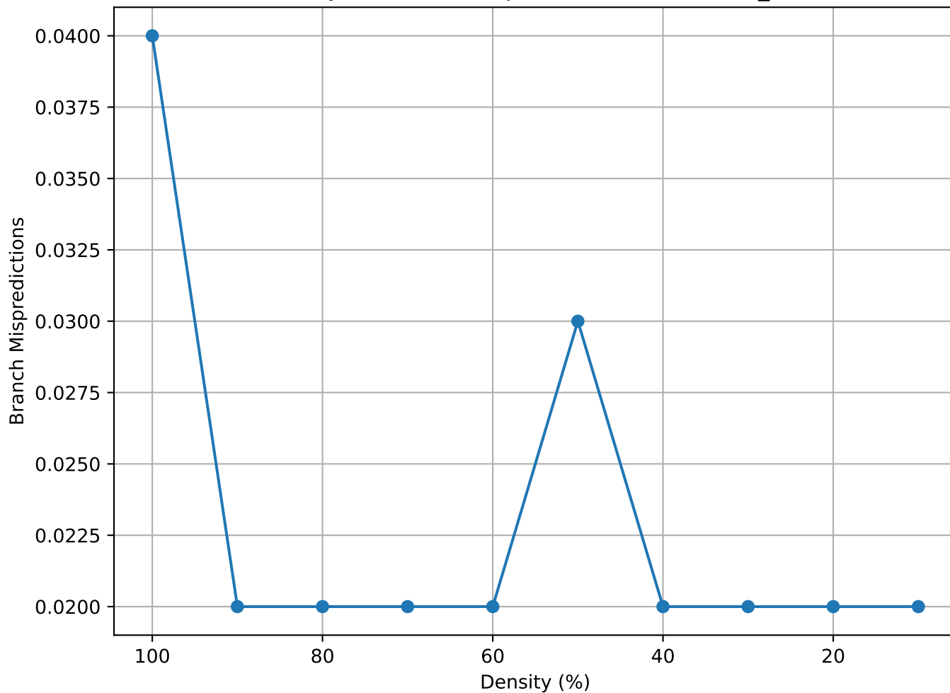
Matrix Density vs Branch Mispredictions (lowThrust_9 - consec)
