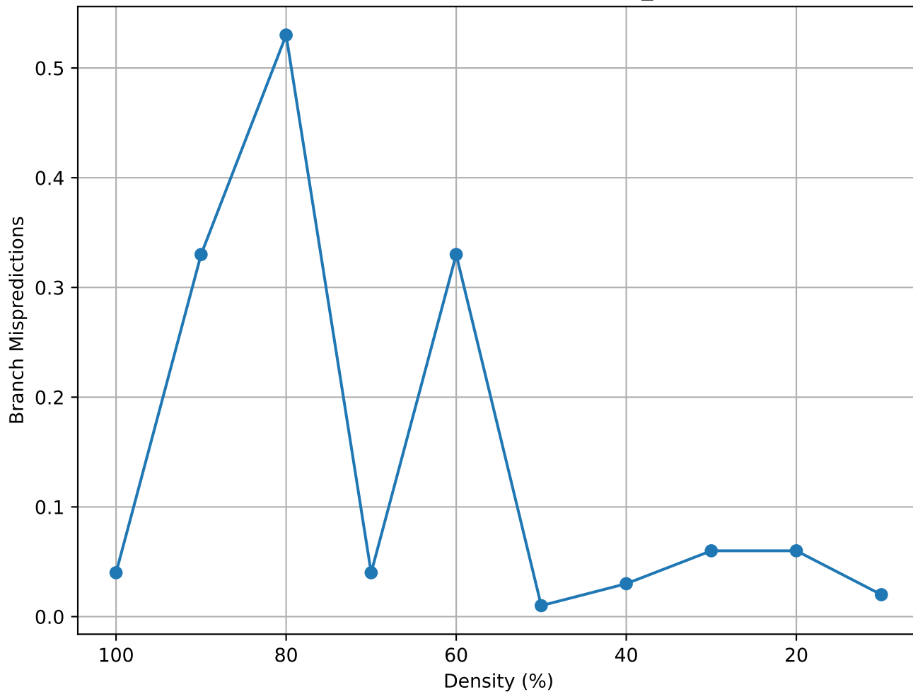
Matrix Density vs Branch Mispredictions (lp_fit2p - truncated)
