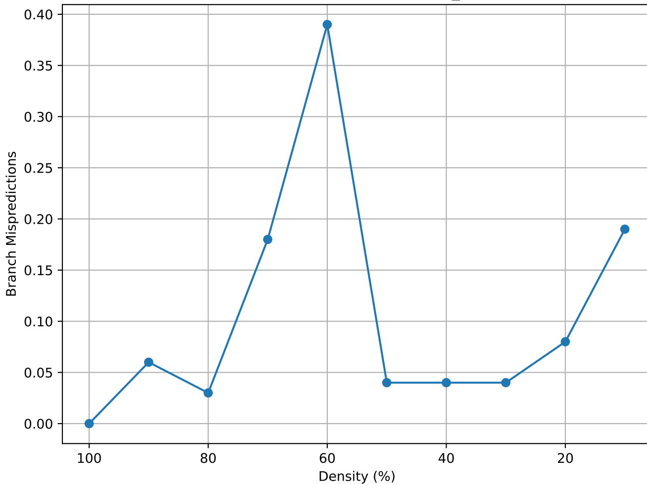
Matrix Density vs Branch Mispredictions (lp_wood1p - random)
