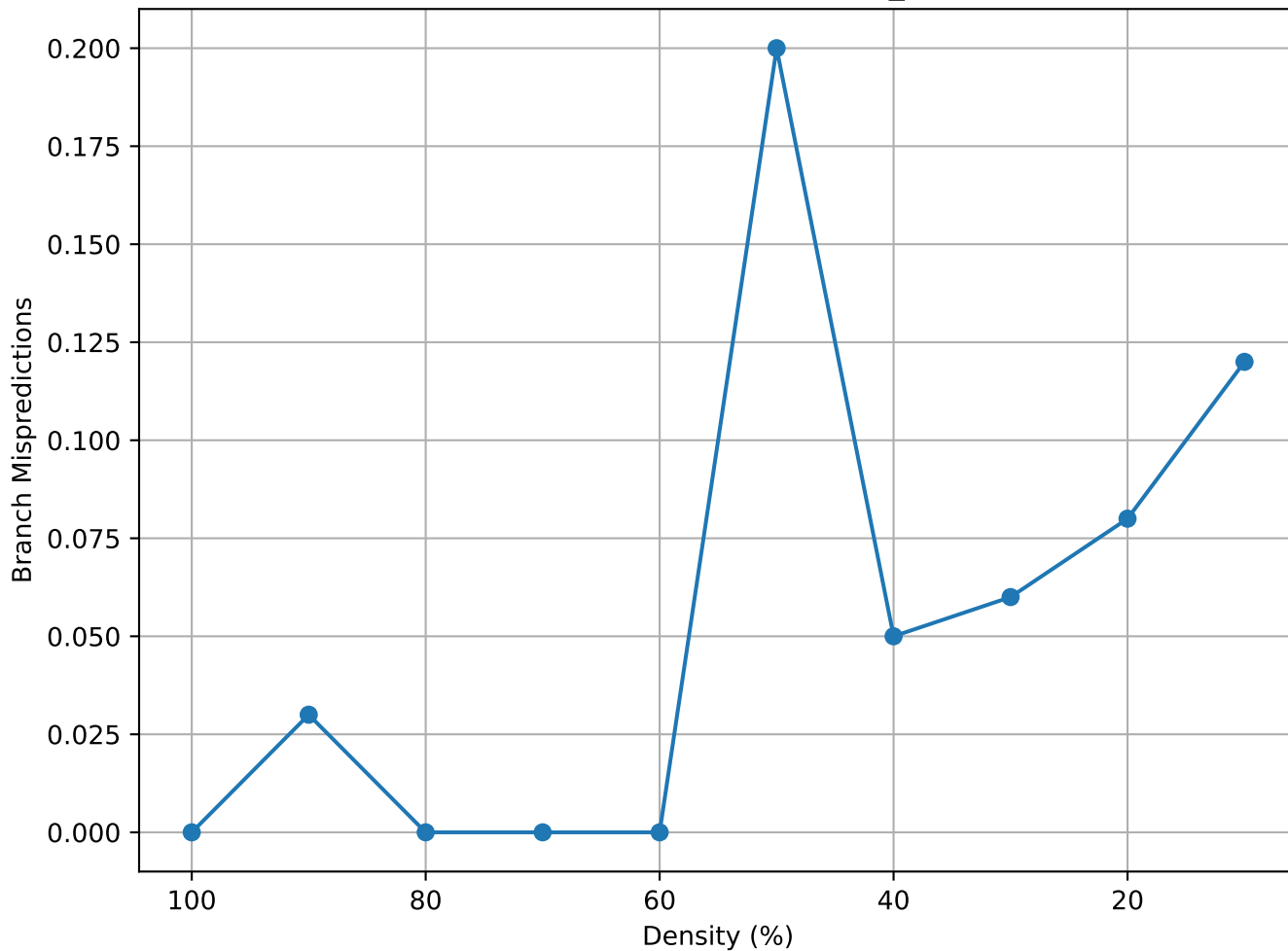
Matrix Density vs Branch Mispredictions (lp_wood1p - truncated)
