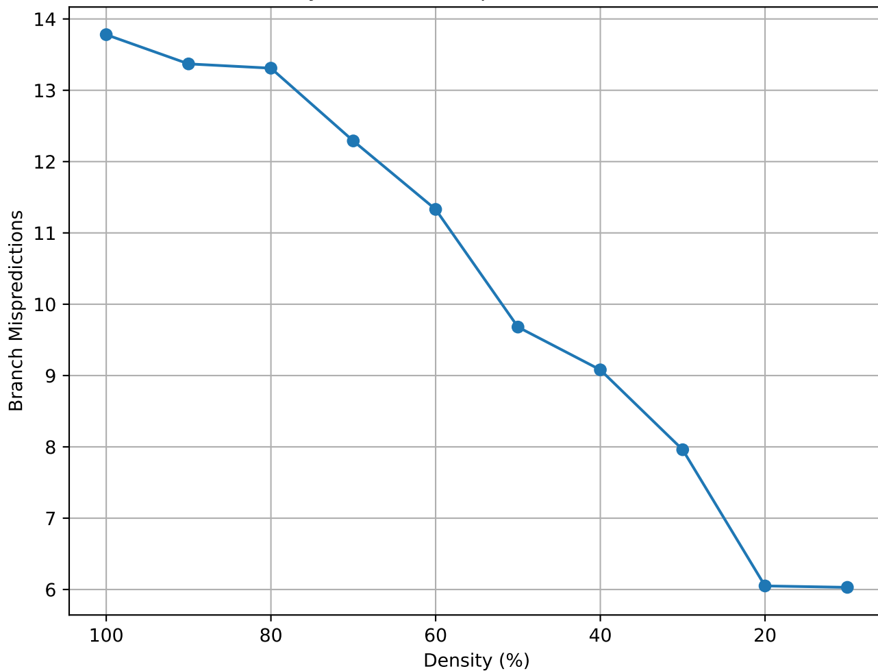
Matrix Density vs Branch Mispredictions (nd12k - consec)
