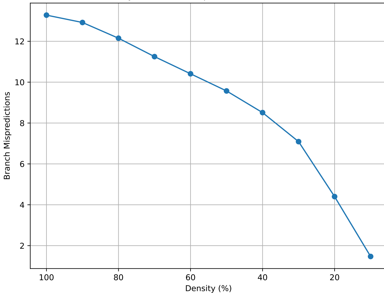
Matrix Density vs Branch Mispredictions (nd12k - truncated)
