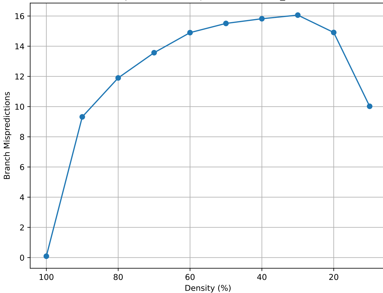
Matrix Density vs Branch Mispredictions (std1_Jac2 - random)
