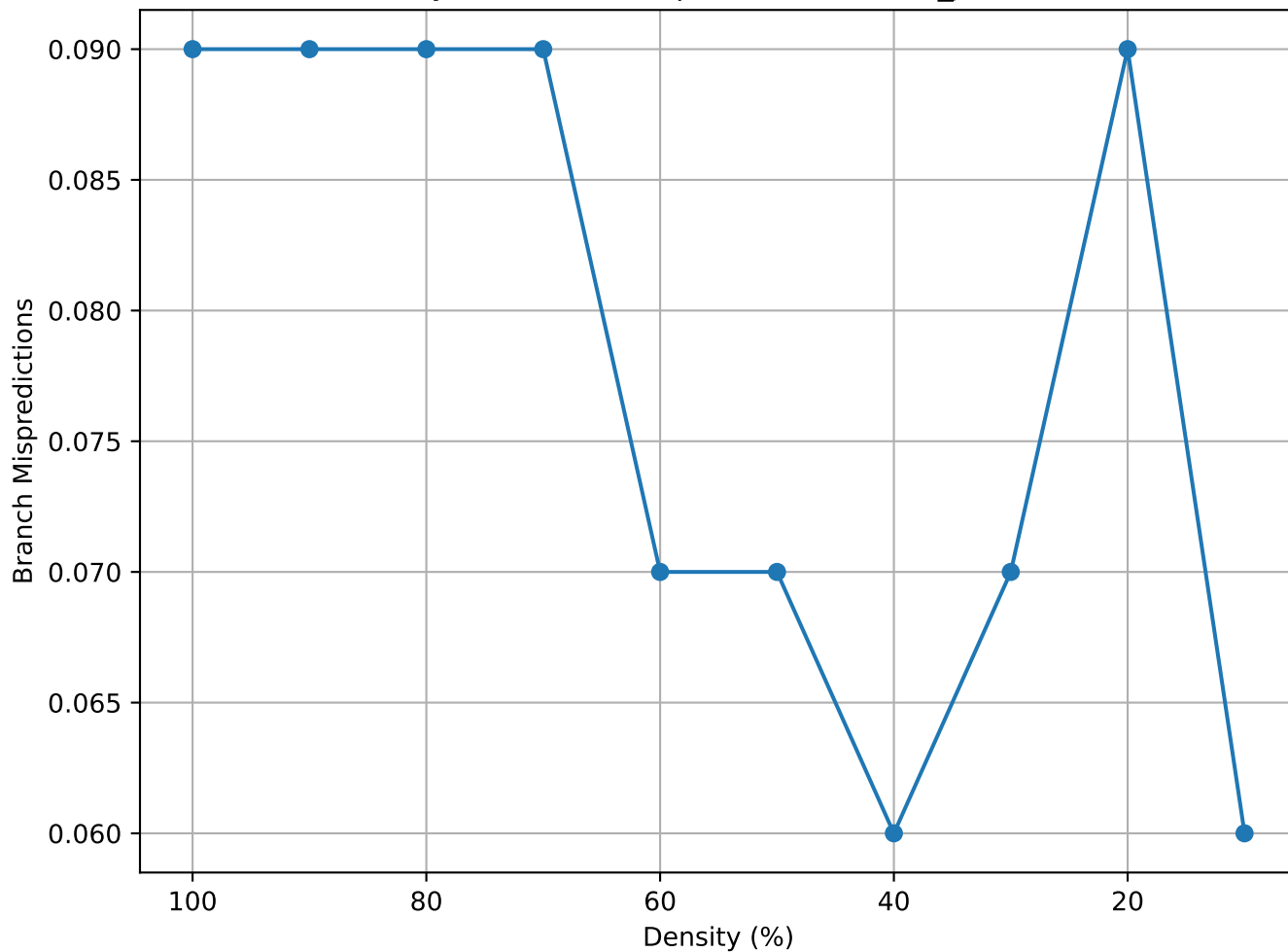
Matrix Density vs Branch Mispredictions (std1_Jac2 - truncated)
