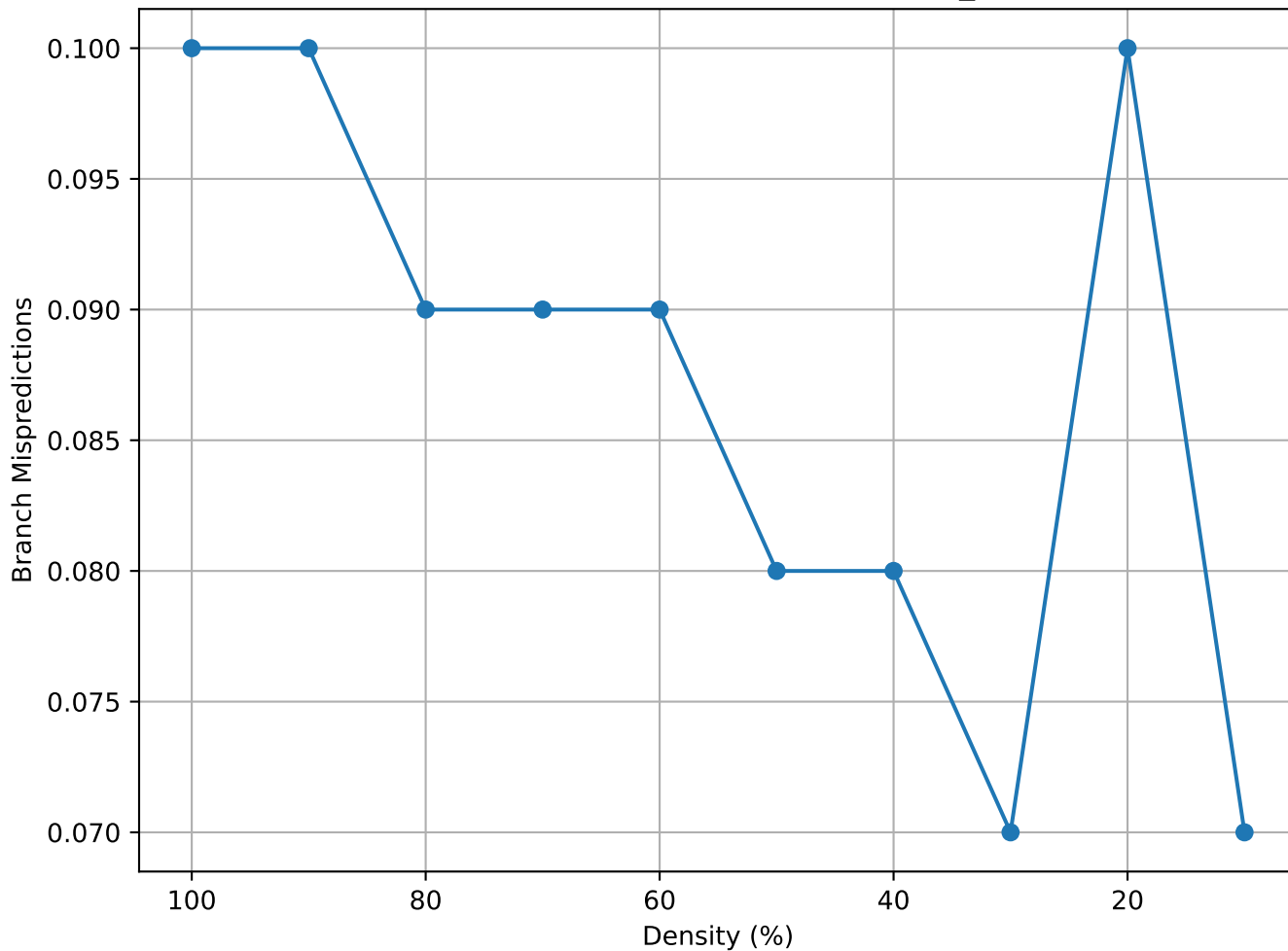
Matrix Density vs Branch Mispredictions (std1_Jac3 - consec)
