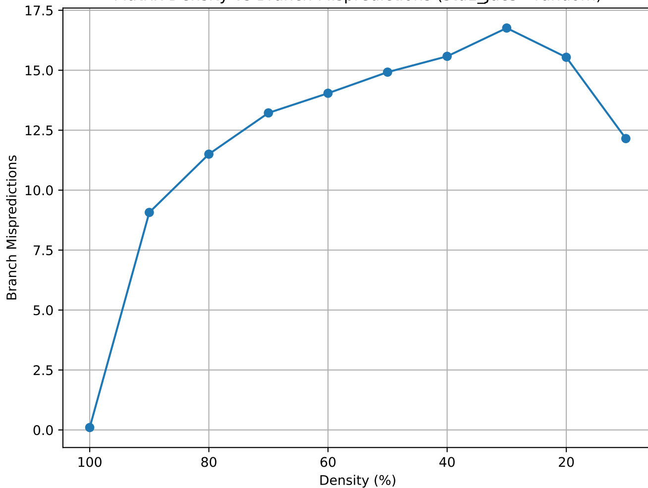
Matrix Density vs Branch Mispredictions (std1_Jac3 - random)
