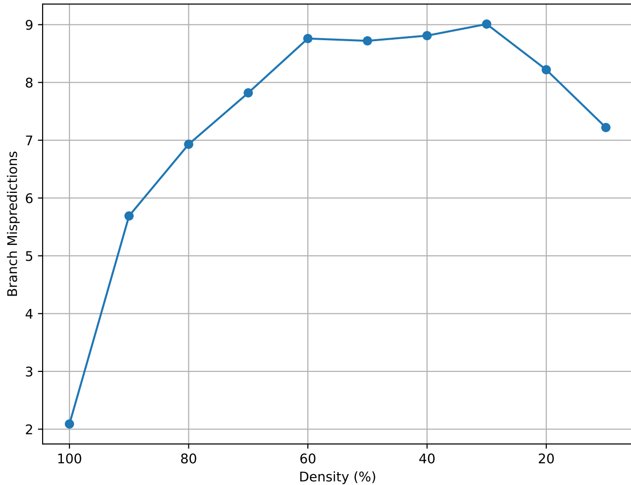
Matrix Density vs Branch Mispredictions (vsp_c-30_data_data - random)
