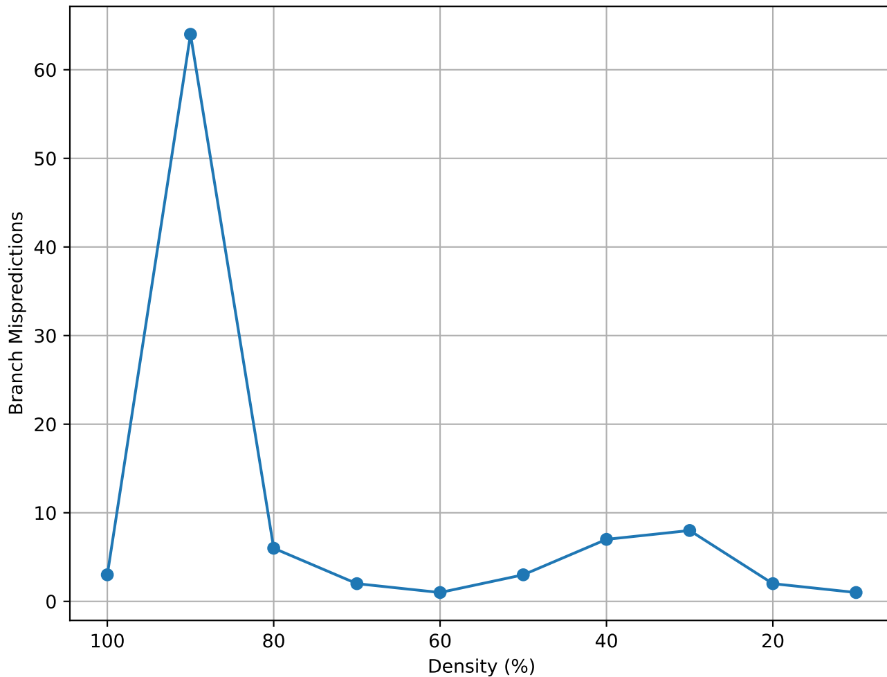
Matrix Density vs Branch Mispredictions (G27 - truncated)
