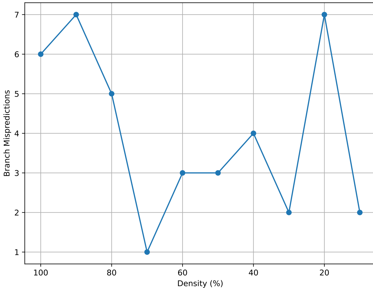
Matrix Density vs Branch Mispredictions (G39 - truncated)
