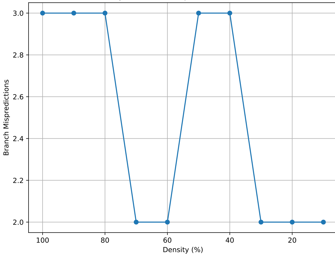
Matrix Density vs Branch Mispredictions (Sieber - consec)
