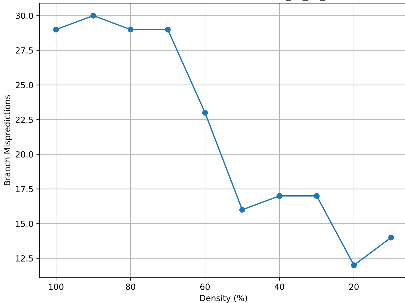
Matrix Density vs Branch Mispredictions (TSOPF_FS_b9_c6 - truncated)
