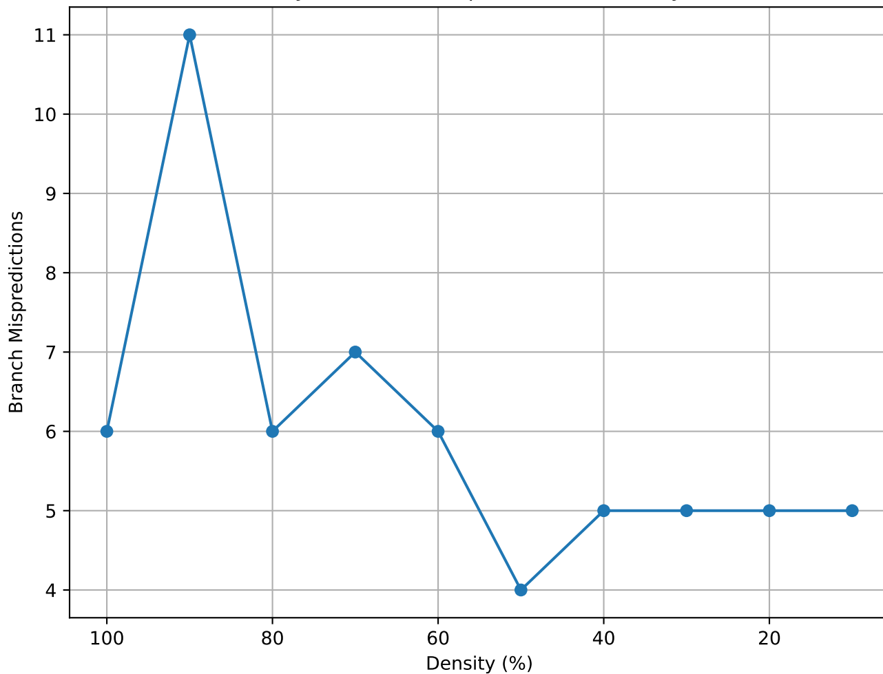
Matrix Density vs Branch Mispredictions (bloweybl - consec)
