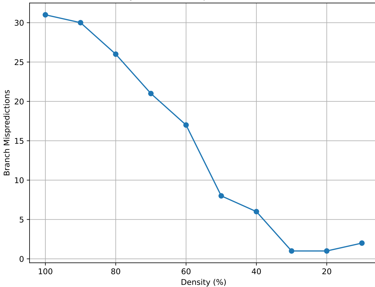
Matrix Density vs Branch Mispredictions (c-30 - truncated)
